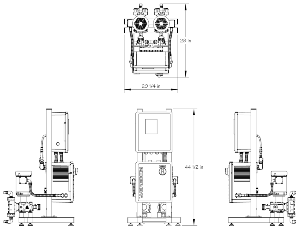
BASE CHASSIS DRAWING - ACTUAL LAYOUT MAY VARY.
